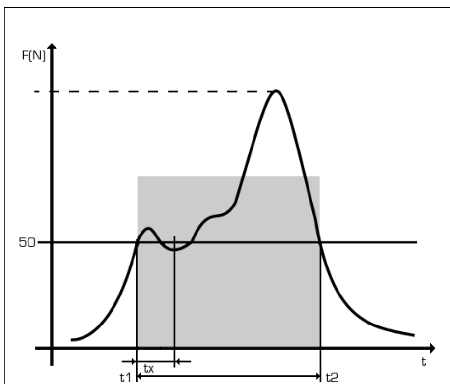
Figure: Force impulse at the beginning of a closing process
