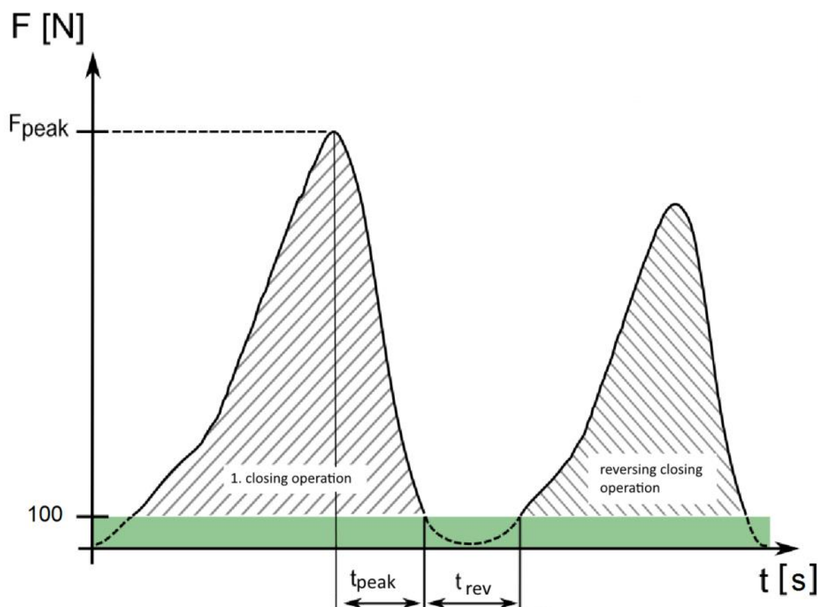
The closing process according EN 14752:2020
